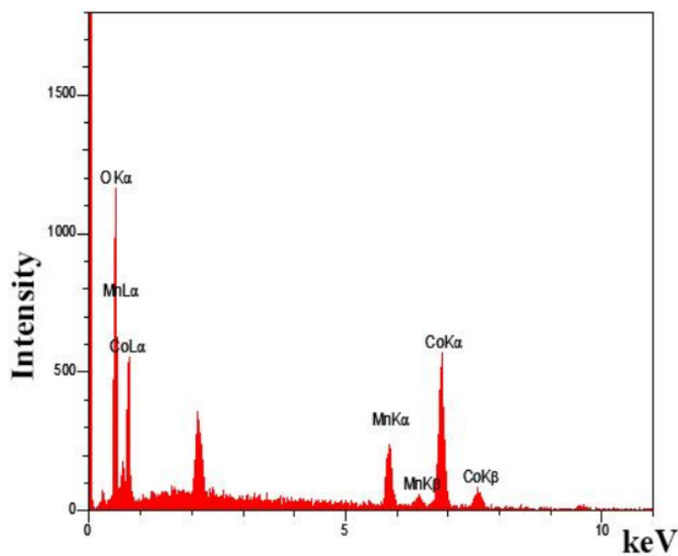
Fig. 3. EDS spectrum of MnCo 2 O 4 /Co 3 O 4 Nanocomposites prepared at 10 min in 900 W.
