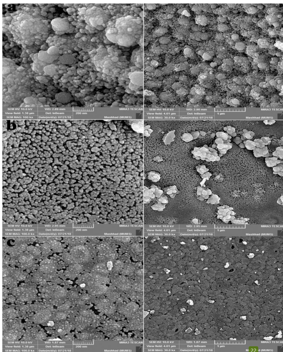
Fig. 4. SEM images of the MnCo 2 O 4 /Co 3 O 4 samples synthesized with different condition in two magnification: (a) 10 min at 750 W, (b) 10 min at 900 W, (c) 10 min at 900 W cyclic reaction (1min on 30 sec off).
