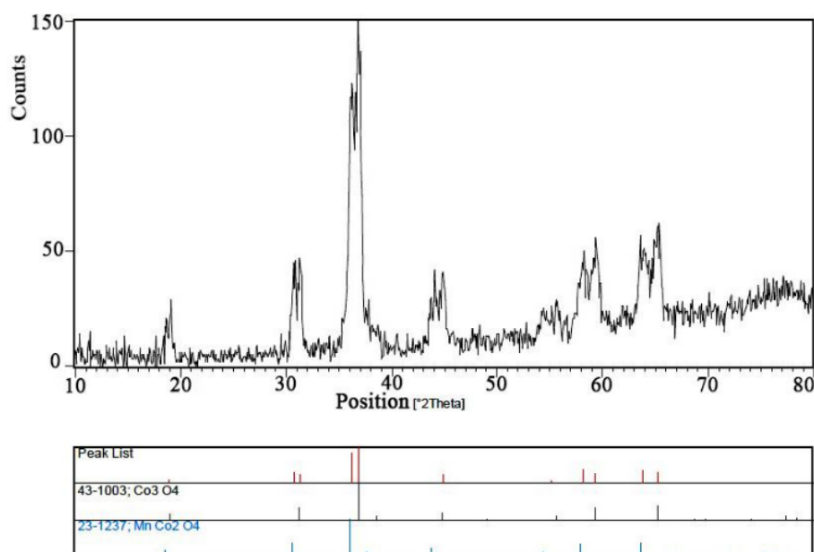
Fig. 1. XRD pattern of MnCo 2 O 4 /Co 3 O 4 Nanocomposites prepared at 10 min in 900 W.
