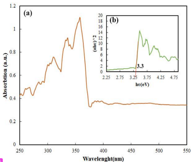
26 Fig. 6. (a) UV-Vis diffuse reflectance spectrum (DRS) of the MnCo 2 O 4 /Co 3 O 4 Nanocomposites prepared at 10 min in 900 W, and (b) the plot of (\alpha h\nu)^2 against h\nu to determine the band gaps.
