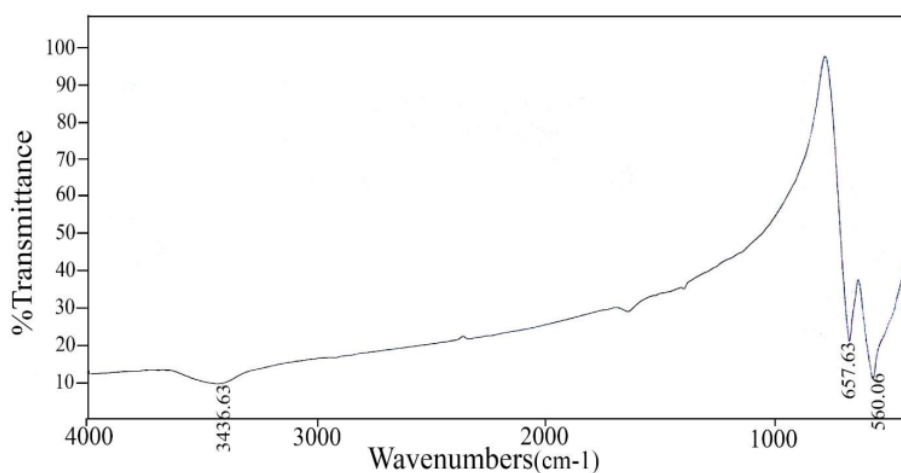
Fig. 2. FT-IR spectrum of MnCo 2 O 4 /Co 3 O 4 Nanocomposites prepared at 10 min in 900 W.
