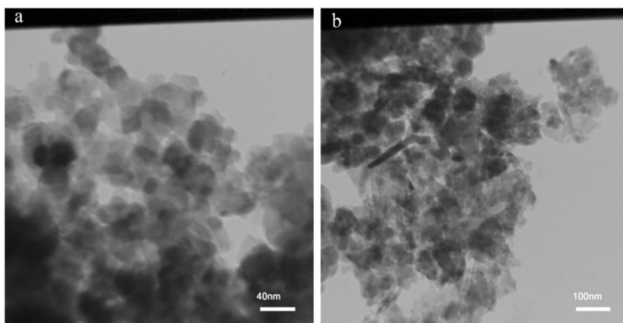
Fig. 5. TEM images of the MnCo 2 O 4 /Co 3 O 4 Nanocomposites prepared at 10 min in 900 W
