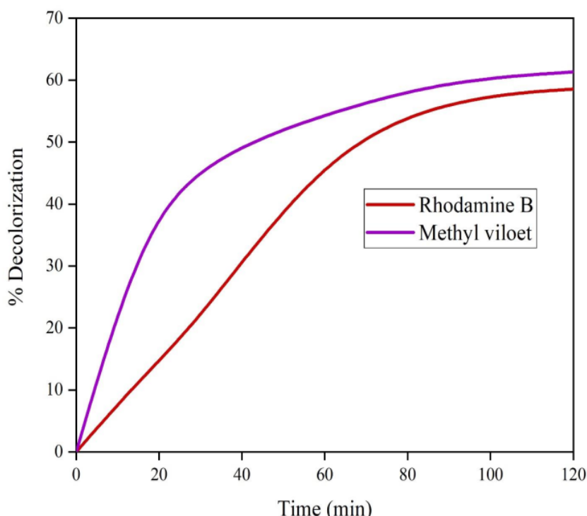
Fig. 7. Photocatalytic activity of MnCo 2 O 4 /Co 3 O 4 nanocomposites against the rhodamine B and methyl violet
